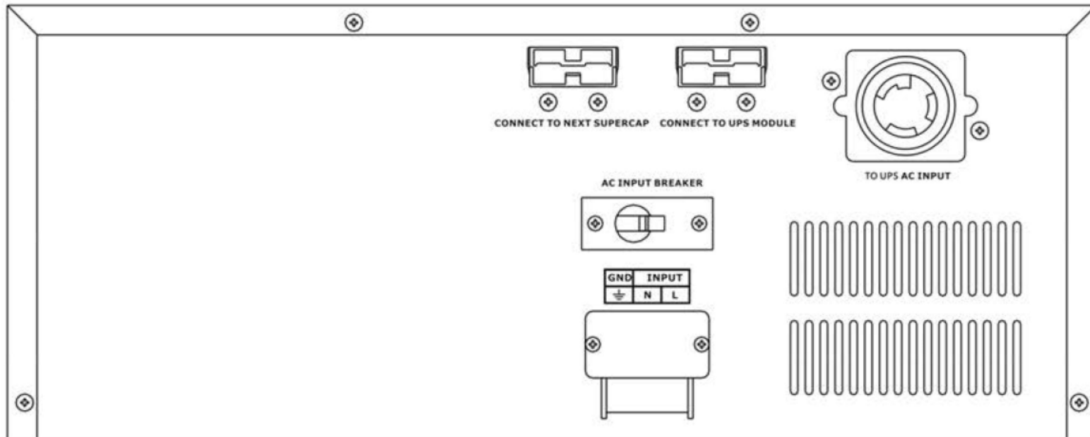
Energy Storage Module Part Number: ARTE-3000-H1
